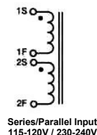
Primary Schematics
